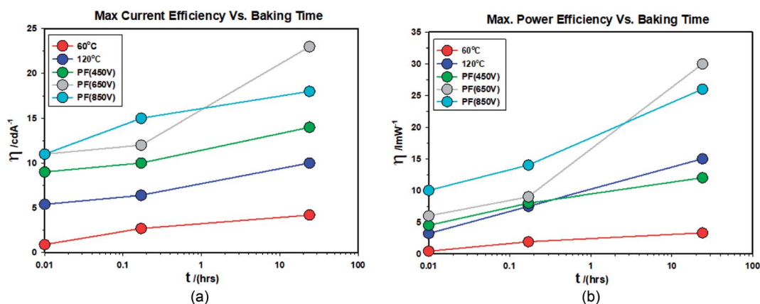
Fig. 19 (a) Maximum current efficiency (left) and (b) maximum power efficiency (right) at 1000 \text{ cd m}^{-2} for devices comprising ZnO (120 °C), ZnO (60 °C), ZnO (60 °C) + PF (450 V), ZnO (60 °C) + PF (650 V) and ZnO (60 °C) + PF (850 V). C1: t = 0 , C2 = 10 minutes, C3: 24 hours.
