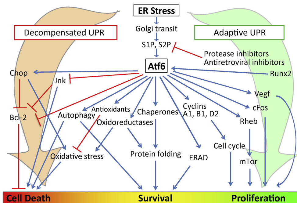
Figure 2: Summary of ATF6 \alpha -regulated pathways regulating cell fate decisions leading to cell death, cell survival or proliferation. S1P, site 1 protease. S2P, site 2 protease. Chop, C/EBP homologous protein. Jnk, c-Jun N-terminal kinase. Runx2, Runt-related transcription factor 2. Bcl-2, B-cell lymphoma 2. Vegf, Vascular endothelial growth factor. cFos, human homolog of Finkel–Biskis–Jinkins murine osteogenic sarcoma virus oncogene. Rheb, Ras homolog, mTor binding. ERAD, ER associated degradation. mTor, mammalian target of rapamycin. Please see the text for citations.
