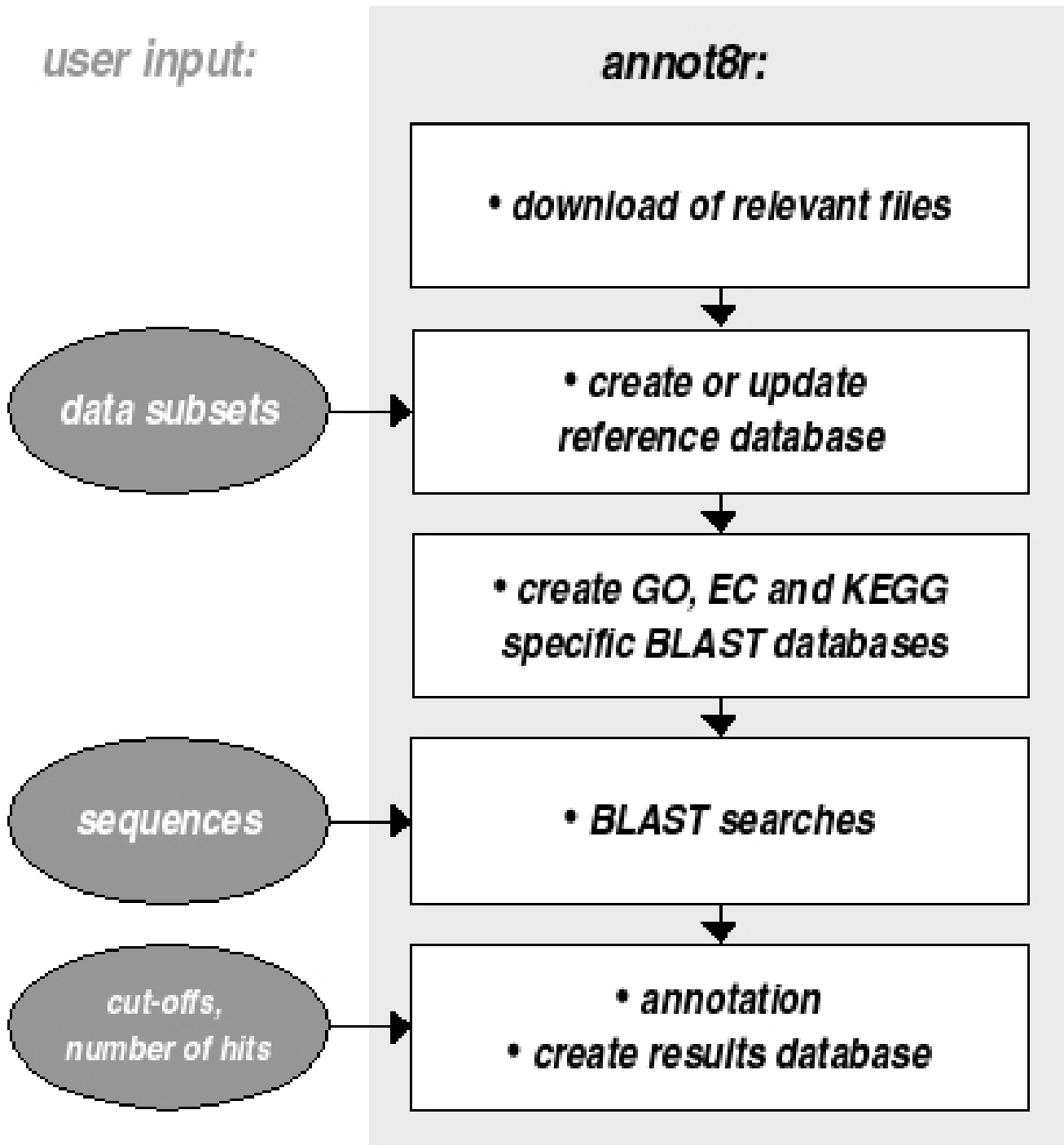
Figure 1 Overview of annot8r . The figure describes the data flow for the five main annot8r steps and indicates where, and what type of, user input is required. For the analysis of multiple datasets steps one to three need only be performed once, as they prepare the reference databases for the annotation process. However, we recommend updating the reference databases from time to time to take advantage of the most recent information available.
