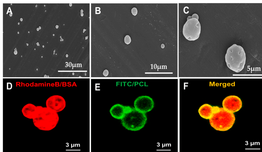
Figure 2. SEM images of bFGF-PCL-MS with three different magnifications (A) 2400 \times (B) 6500 \times and (C) 10,000 \times . Confocal microscopy images of fluorescent PCL-MS. (D) RhodamineB/BSA distribution in the microspheres. (E) FITC/PCL distribution in the microspheres. (F) Merged image.
