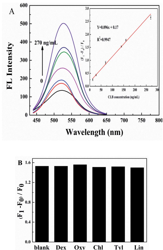
Fig. 5 (A) Fluorescence spectra of G-CDs with 3.0 nM AuNPs nano-sensor in the presence of different CLB at increased concentration: 0, 13, 28, 70, 140, 160, 270 ng mL -1 . Inset: calibration plot for CLB. (B) Fluorescence recovered efficiency of G-CDs–AuNPs–CLB in the presence of other substances, the concentration of CLB was set as 140 ng mL -1 , B–R buffer pH = 6.0, the Dex, Chl, Tyl, and Lin were 10 times CLB concentration, Oxy was 1 time CLB concentration.
