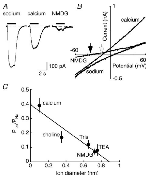
FIGURE 2. Permeation properties of algae P2X receptor. A , whole-cell currents evoked by ATP (1 mM); holding potential -60 mV. Currents were evoked in external solution containing 147 mM sodium chloride, 98 mM calcium chloride, and 148 mM N -methyl-D-glucosamine; chloride (NMDG). B , current-voltage plots for ATP-evoked currents in external sodium, calcium, or NMDG. Note left shift in reversal potential in calcium (open arrowhead) or NMDG (filled arrowhead). C , permeability of five cations relative to that of sodium as a function of their mean geometric diameter. Points are mean \pm S.E. of the mean; n = 8 cells.
