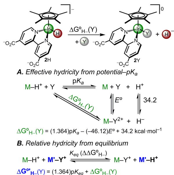
Figure 1. Scheme illustrating the hydricity of reference complex [\text{Cp}^*\text{Ir}(\text{bpy-COO})(\text{H})]^- (2H) and thermochemical cycles that establish aqueous hydricity of Ir and Ru hydrides.
