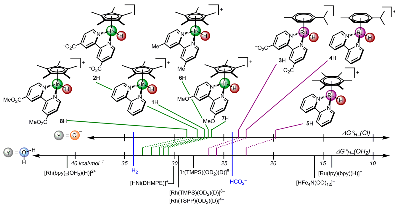
Figure 5. Aqueous hydricity scale of the complexes we report along with those previously reported in the literature. Y represents the incoming ligand such that the top scale shows \Delta G^{\circ}_{\text{H}^-(\text{Cl})} and the bottom scale shows \Delta G^{\circ}_{\text{H}^-(\text{OH}_2)} . TSPP = tetra( p -sulfonatophenyl)porphyrin; TMPS = tetrakis(3,5-disulfatomesityl)porphyrin; tpy = terpyridine; DHMPE = 1,2-bis(dihydroxymethylphosphino)ethane. 19,22,23,49
