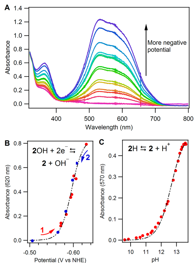
Figure 2. (A) Spectral changes of a pH 14 solution of [\text{Cp}^*\text{Ir}(\text{bpy-COO})(\text{OH})]^- (2OH) as the solution potential is decreased by electrolysis to form [\text{Cp}^*\text{Ir}(\text{bpy-COO})]^{2-} (2). (B) Absorbance at 620 nm stepping in the negative potential direction (red dots), the positive potential direction (blue dots), and the fit to the Nernst equation (dot-dashed line) giving E^{\circ'} = -0.60 V. The lack of hysteresis indicates that equilibrium was established. (C) Absorbance at 570 nm of a pH titration of [\text{Cp}^*\text{Ir}(\text{bpy-COO})(\text{H})]^- (2H) forming 2 (red dots) and the fit to the Henderson–Hasselbalch equation (dot-dashed line) giving pK_a = 12.4 .
