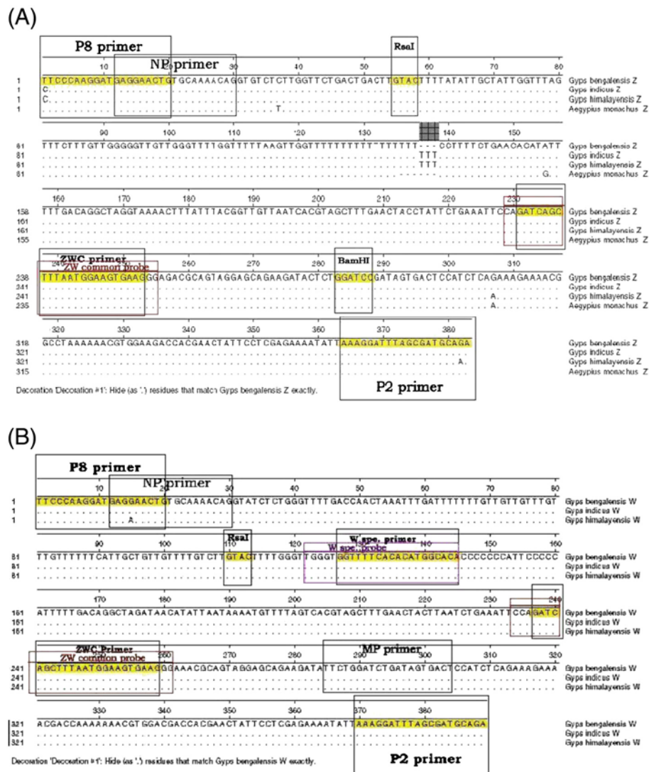
Figure 1 Sequence alignment of CHD-Z and CHD-W allele sequences amplified by Griffith's universal CHD primer pair P2/P8 in four species of vultures ( Gyps bengalensis , Gyps indicus , Gyps himalayensis , Aegypius monachus ) by ClustalW (MegAlign DNASTar). The sequences of primers P2, P8, NP, MP, ZW common primer and probe, W-specific primer and probe recognition sites; Bam HI and Rsa I restriction sites are boxed. (---) Dashed lines indicate sequence similarity. A. ) Alignment of CHD-Z sequences. B. ) Alignment of CHD-W sequences.
