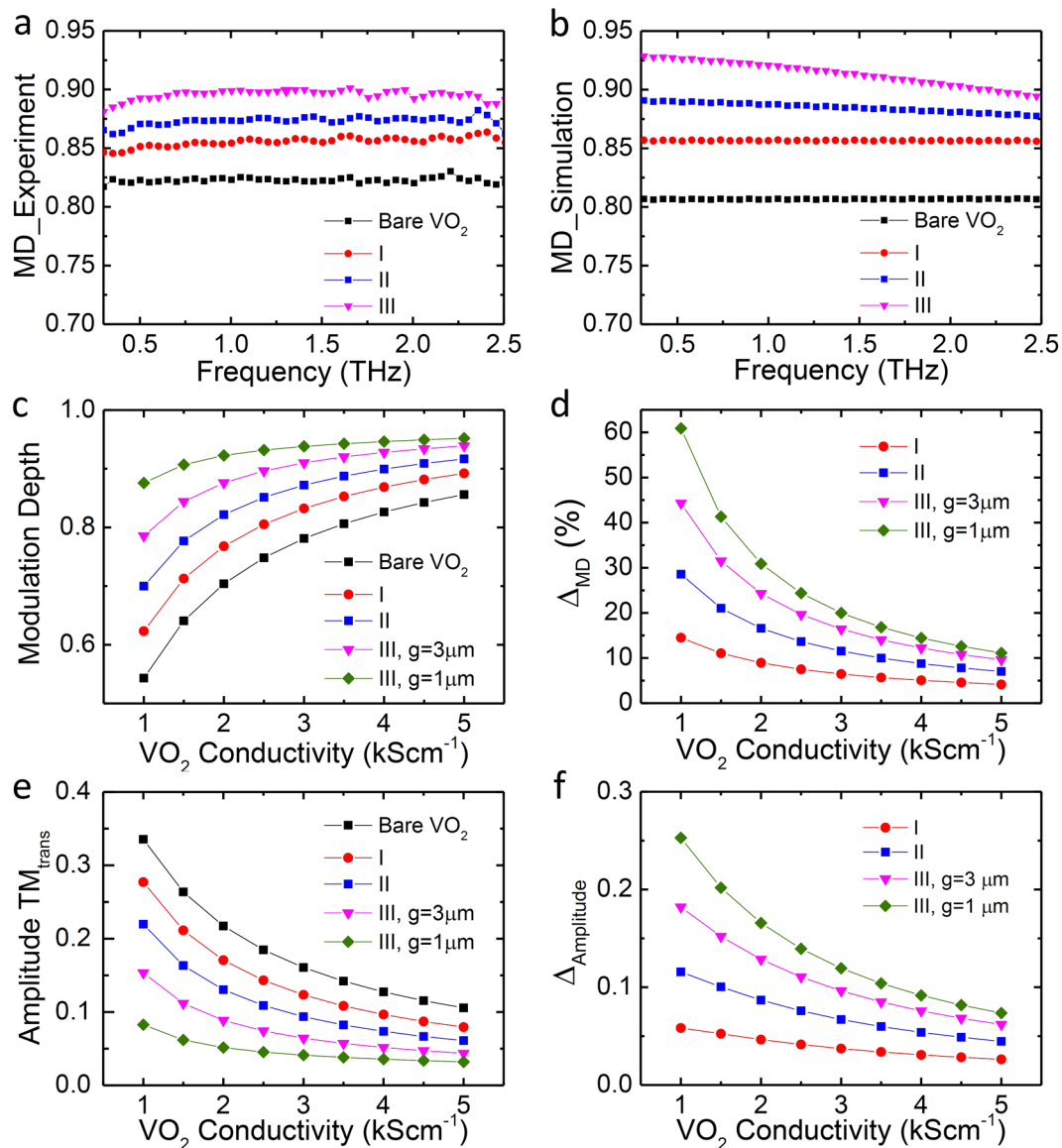
Figure 3. Modulation depth characterization. (a) The experimental modulation depth for bare VO 2 by thermal activation (black squares), sample I (red dots), sample II (blue squares) and sample III (pink triangles) by electrical activation. (b) The corresponding simulated MD. (c) Simulated modulation depth at 1 THz for bare VO 2 (black squares), sample I (red dots), sample II (blue squares), sample III with g = 3 \mu\text{m} (pink triangles) and 1 \mu\text{m} (green diamonds), respectively, as a function of VO 2 conductivity. (d) Increase in MD for different types of sample compared to bare VO 2 . (e) Simulated TM amplitude transmission at 1 THz as a function of VO 2 conductivity. (f) Decrease in amplitude transmission for different types of sample compared to bare VO 2 at 1 THz as a function of VO 2 conductivity.
