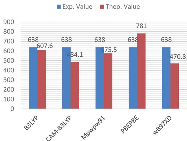
Fig. 2 Comparison diagram of \lambda_{\max} value of R with \omega B97XD, B3LYP, CAM-B3LYP, PBEPBE and MPW1PW91 at 6-31G(d,p).
