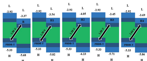
Fig. 9 The open circuit voltages ( V_{oc} ) of reference R and H1 – H4 with respect to donor material PBDB-T donor.
