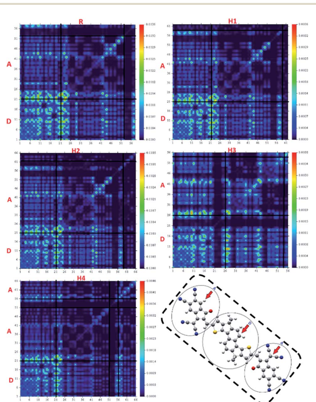
Fig. 10 Transition density matrix of reference R and designed molecules ( H1 – H4 ) at S_1 state.
