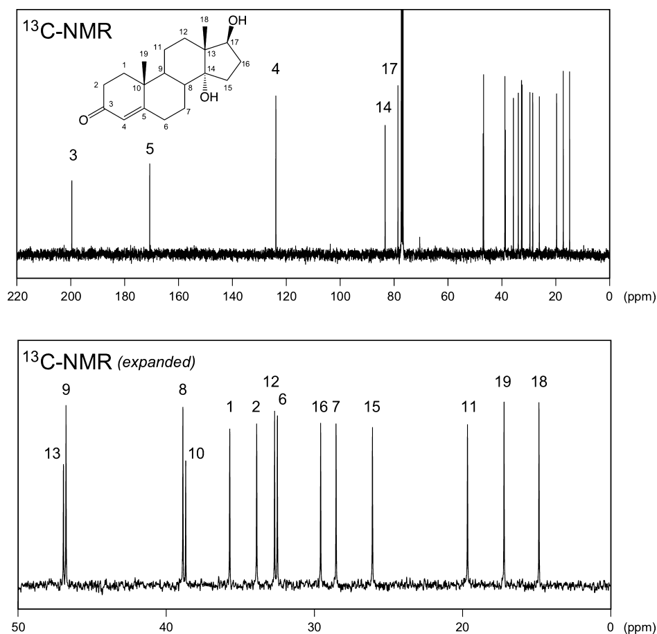
Figure 2. 13 C NMR spectra of 14α-hydroxytestosterone produced by CYP5312A4.
