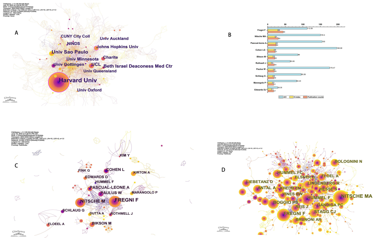
Figure 3 Institutions and authors posting, collaborative contributions (A) CiteSpace visualization of the institutions associated with tDCS treatment for stroke during 2004–2022. (B) The publication counts, H-index, and ACI of the top 10 authors associated with tDCS treatment for stroke during 2004–2022. (C) CiteSpace visualization of the authors associated with tDCS treatment for stroke during 2004–2022. (D) CiteSpace visualization of the co-citation authors associated with tDCS treatment for stroke during 2004–2022.
