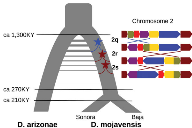
Figure 5. Schematic of the speciation history of D. arizonae and D. mojavisensis . The onset of divergence around 1.3 MY was followed by a prolonged period of gene flow that ceased before the divergence of the different populations of D. mojavisensis . Inversion 2q arose in D. mojavisensis during the onset of divergence (blue star) and is the first in a cascade of three overlapping inversions on chromosome 2 that became fixed in D. mojavisensis (adapted from Guillen and Ruiz (2012)).
