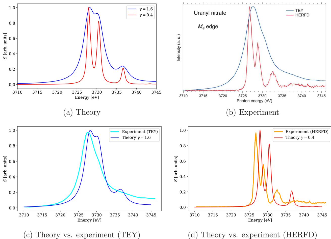
Figure 11. Calculated 4c-DR-TDDFT (PBE0-60HF, VDZ/aVDZ) XAS spectra near the uranium M_4 -edge of UO_2(NO_3)_2 using different damping parameters and their comparison with the experimental results. 122 The spectra were normalized by setting the maximum to unity. (a) Theory and (b) experiment (reprinted from ref 122, copyright 2016 American Chemical Society). (c) Theory vs experiment (TEY); (d) theory vs experiment (HERFD).
