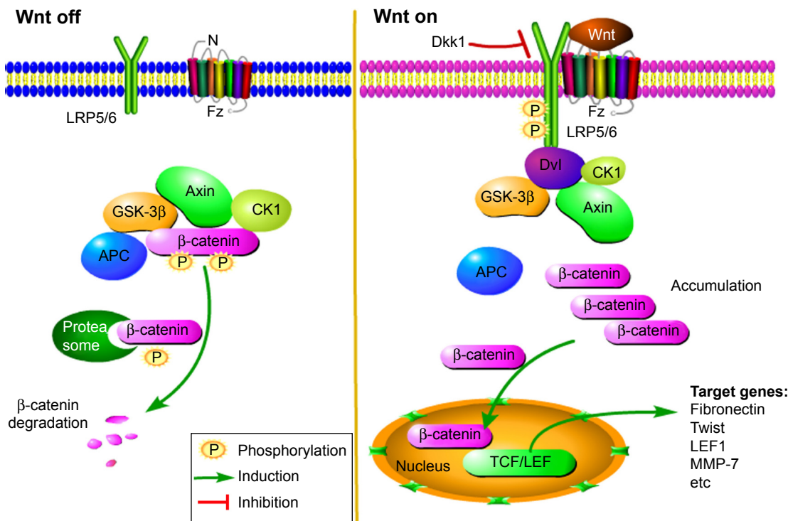
Figure S1 Simplified schematic of the canonical Wnt/ \beta -catenin signaling pathway.
