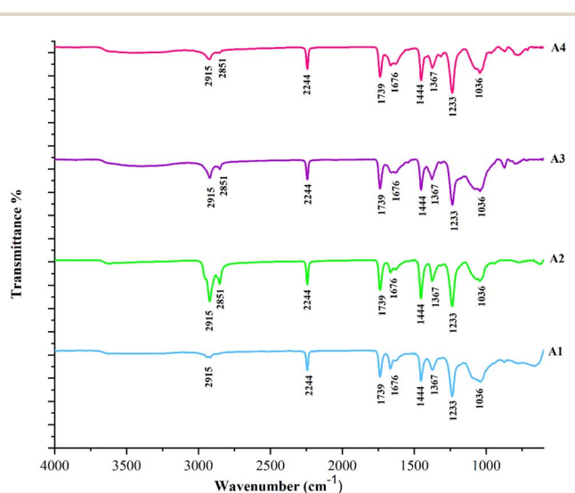
Fig. 3 FTIR spectra of developed adsorbents (A1, A2, A3, and A4).
