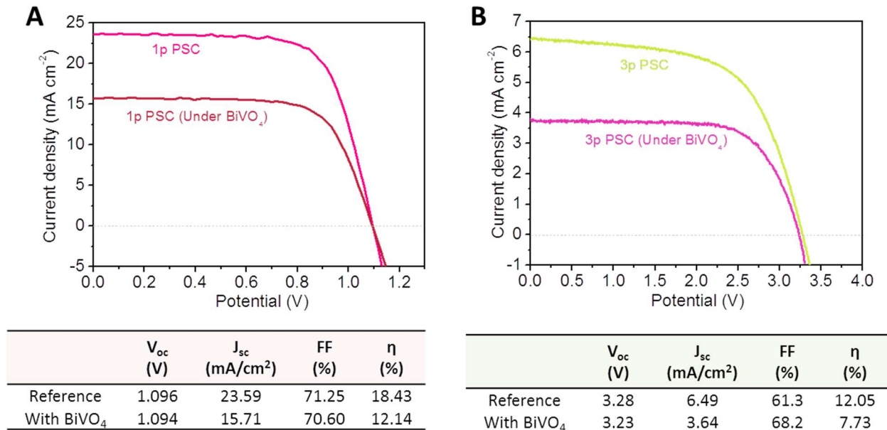
Figure S19. Performance of lead halide based perovskite PV, related to Figure 5. J-V curves of (A) single piece and (B) 3 pieces PSCs connected in series with/without the overlay of NiFeO x /H, 1% Mo:BiVO 4 PE. Inset table indicates performance of devices. Light intensity was 1 sun (AM 1.5G, 100 mW/cm 2 ).
