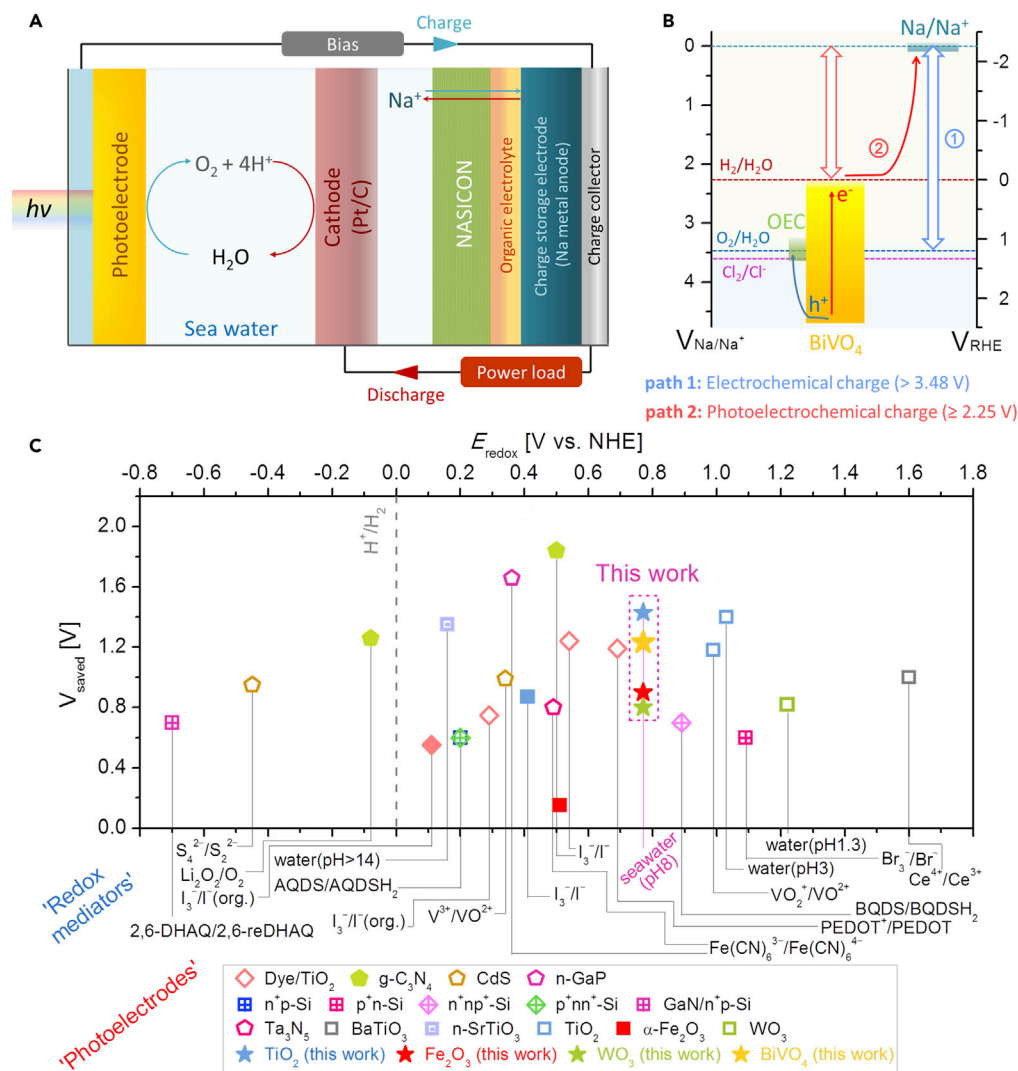
Figure 1. Cell Configuration and Photo-charging Process of the Solar Seawater Battery (A) The cell structure of a solar rechargeable seawater battery, which employs a NASICON ceramic membrane to separate a charge storage electrode (Na metal anode) from a photoelectrode (PE) and a cathode immersed in seawater. (B) Energy diagram of the photo-charging process, where OEC-loaded BiVO 4 PE is employed for solar seawater oxidation at the cathode compartment. The energy level is expressed with two different scales relative to reversible hydrogen electrode (RHE) of seawater (pH~8) and the redox potential of Na/Na + . The PEC seawater splitting on the PE significantly reduces the potential required for battery charging (path 1 versus path 2). (C) Redox potential ( E_{\text{redox}} )-voltage saved ( V_{\text{saved}} ) plot of various types of solar rechargeable batteries using redox mediators from literatures. The V_{\text{saved}} was calculated by subtracting the conduction band edge ( E_{\text{CB}}/e ) of photoelectrodes from the E_{\text{redox}} of redox mediators.
