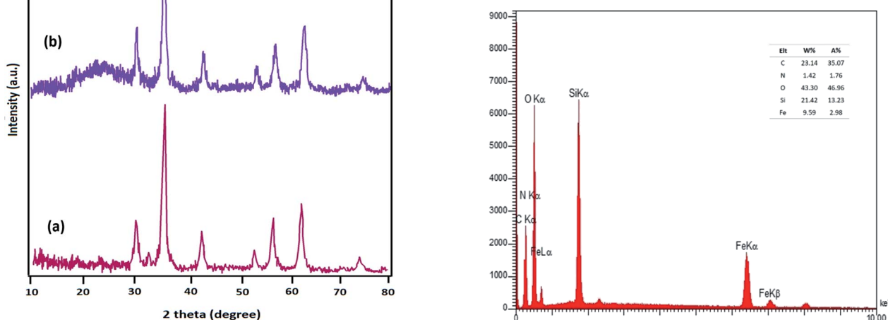
Fig. 2 XRD patterns of (a) Fe 3 O 4 , and (b) Fe 3 O 4 @SiO 2 -L-tryptophan.
