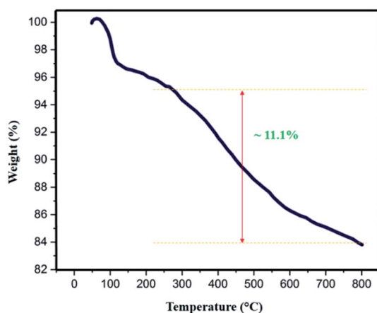
Fig. 7 TGA curve of \text{Fe}_3\text{O}_4@SiO_2 -L-tryptophan NPs.
