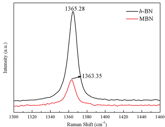
Fig. 7 Raman spectra of h-BN and MBN.
