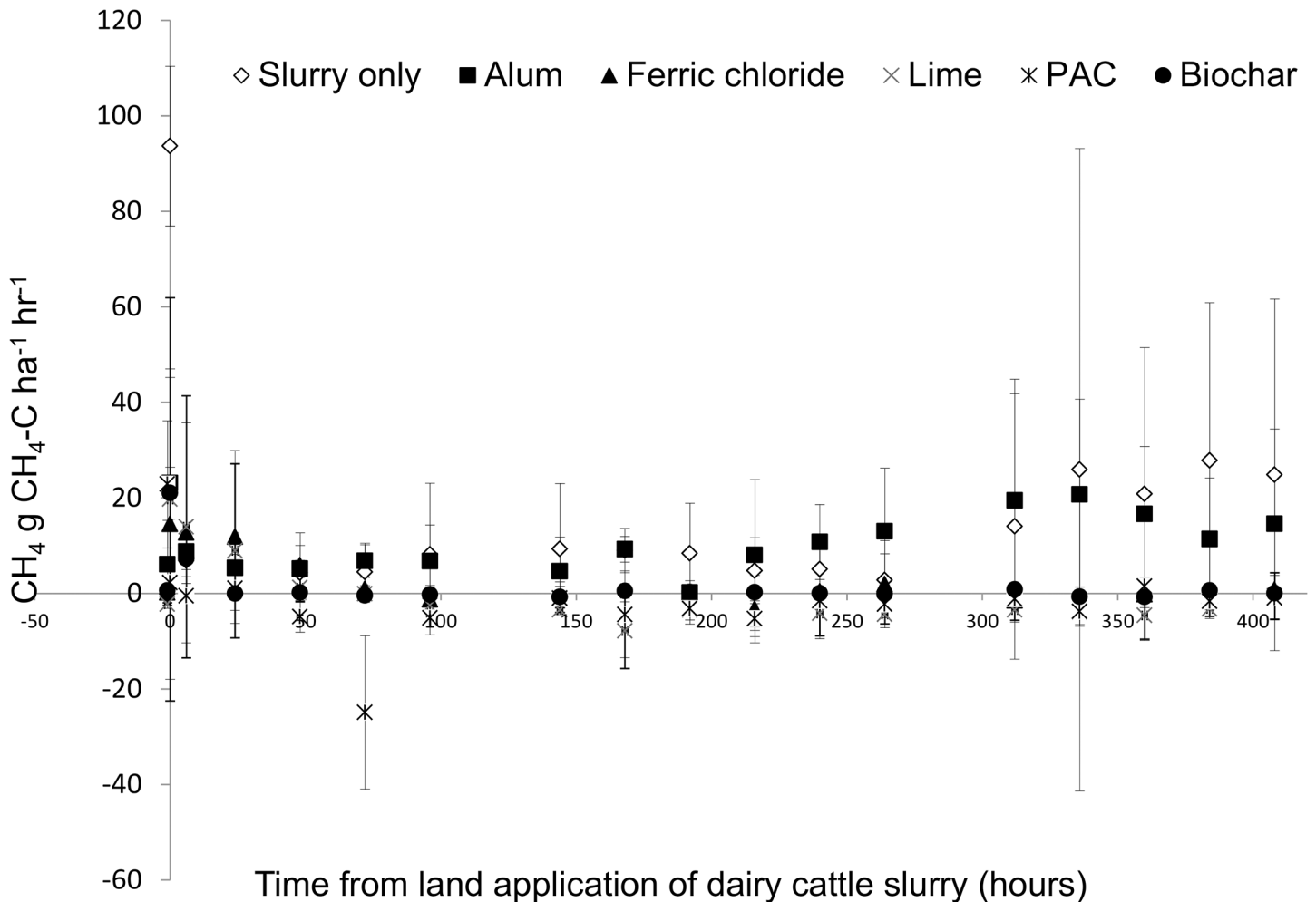
Fig 6. Methane emissions profile. Temporal profile of methane (CH 4 -C) emissions from amended slurry and control treatments for 15 days after application.
