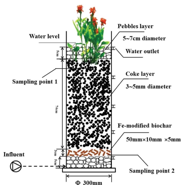
Fig. 1 Schematic diagram of the CW3.
