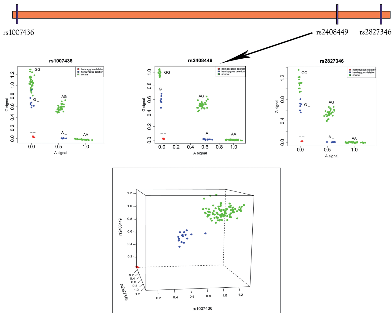
Figure 5. Calling SNP/CNV alleles from raw data. All three SNPs shown here on chromosome 21 have alleles A and G. All plots show A allele and G allele intensity values from Illumina HumanHap550 data for 112 HapMap samples. The top three panels show each of the three SNPs individually along with their generalized genotypes. The bottom panel shows the total raw copy number sums (A signal + G signal) plotted, with each axis representing one of the SNPs. Note that the samples clearly separate into homozygous deletions (red), hemizygous deletions (blue), and normal (green).
