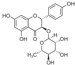
Fig. 1. Chemical structure of engeletin.
