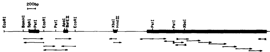
FIGURE 2. Restriction map of the human MBP gene ( \sim 7 kb in length). The thickened lines correspond to exons (14). The arrows indicate the direction and extent of sequence analysis by the dideoxy nucleotide chain termination method utilizing either single-stranded M13 vectors or double-stranded pUC vectors.
