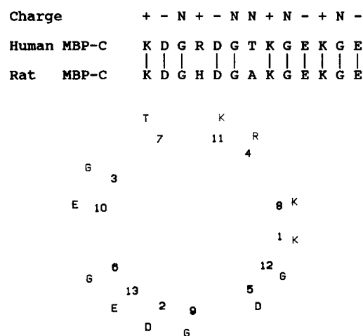
FIGURE 4. Alignment of like-charged amino acids of human MBP-C and rat MBP-C reveals that the positively charged amino acids can be aligned on one face of an \alpha helix with neutral and negatively charged amino acids on the other face, as depicted by a helical wheel. We would like to thank Dr. Jiri Novotny for the helical wheel diagram.
