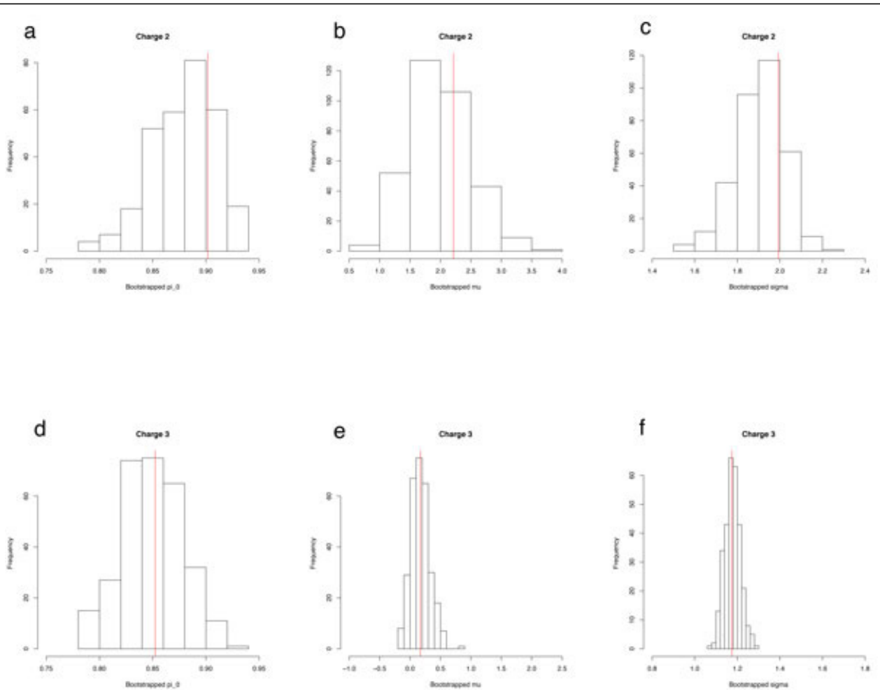
Figure 3 Bootstrapped samples of \pi_0 , \mu , and \sigma for Charges 2 and 3 of the Human Plasma data. The original estimates are marked by the vertical line. The length of the horizontal axes are equal for the plots of a particular parameter. The Charge 2 distributions are slightly skewed compared to Charge 3 distributions and the mean squared errors are much greater in Charge 2 distributions. The variability of the Charge 2 distributions are visibly much greater indicating unstable estimates.
