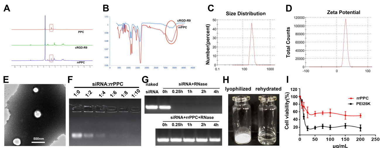
Figure I Characterization of rrPPC/siRNA complex. (A) ^1\text{H} NMR spectra of rrPPC; (B) FT-IR spectra of rrPPC; (C) size distribution of rrPPC nanoparticles; (D) zeta potential distribution of rrPPC nanoparticles; (E) transmission electron microscopy images; (F) gel retardation assay of rrPPC/siRNA complex; (G) RNase degradation assay; (H) rehydration of lyophilized rrPPC powder; and (I) cytotoxicity as evaluated by MTT assay.
