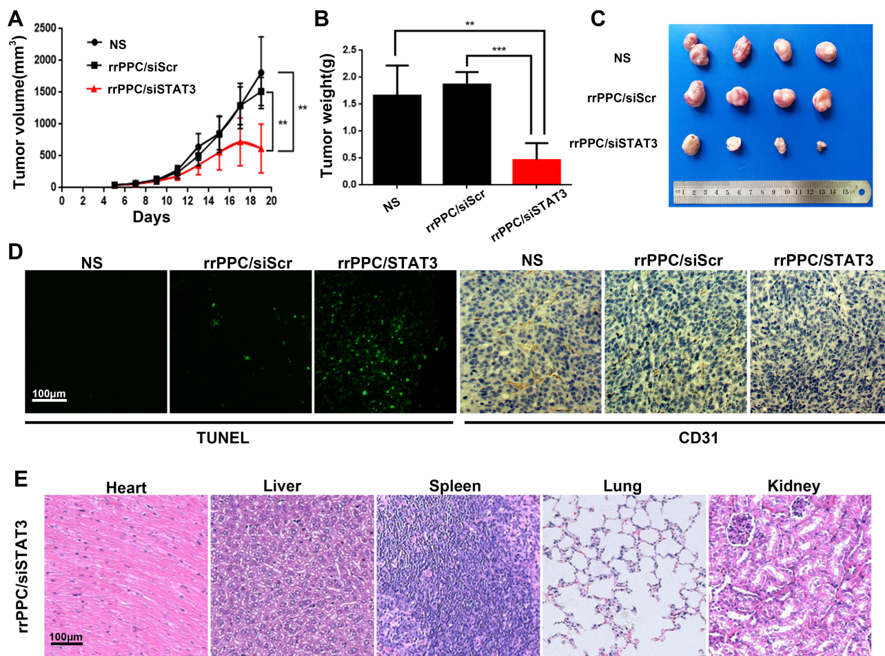
Figure 6 rrPPC/siSTAT3 complex inhibited subcutaneous xenograft tumor growth in vivo. (A) Tumor growth curves of each group (** P < 0.01 ); (B) average tumor weight of each group; (C) representative images of subcutaneous tumor tissues (** P < 0.01 ; *** P < 0.001 ); (D) detection of vessel formation and apoptosis by CD31 staining and TUNEL assay; (E) H&E analysis.
