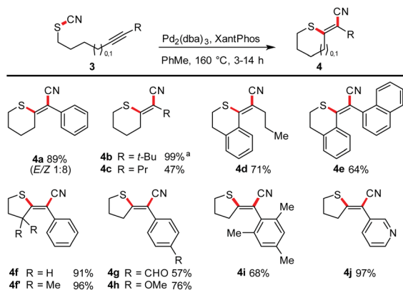
Scheme 4 Intramolecular cyanosulfenylation with aliphatic thiocyanates. Reaction conditions: 3 (1.00 equiv.), Pd 2 (dba) 3 (10 mol%), XantPhos (20 mol%), PhMe (20 mM), 160 °C, 3–14 h. a Pd(PPh 3 ) 4 (5 mol%), SPhos (20 mol%), 160 °C, 3 h, PhMe (20 mM).
