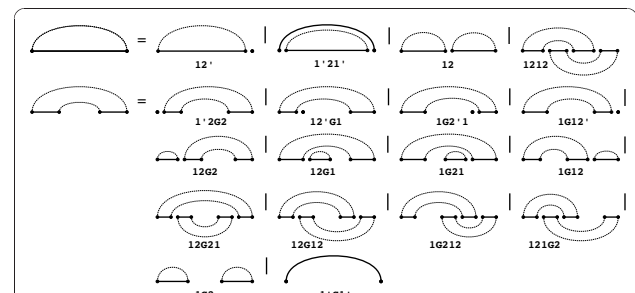
Figure 2 Decomposition for R&E base pair maximization annotated with labels, i.e. split types, of the corresponding recursion cases.
