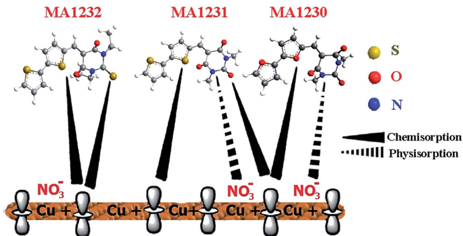
Fig. 13 A schematic diagram of the corrosion protection of Cu dipped in 1 M \text{HNO}_3 corrosion medium with pyrimidine derivatives (MA-1232, MA-1231, and MA-1230).
