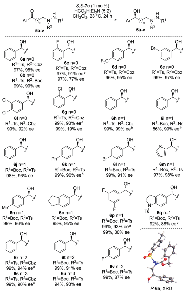
Fig. 2 Ru-catalyzed ATH of hydrazone-containing ketones. a Using R,R -7f. b ee determined after cyclization to 8 . c Using R,R -7c.
