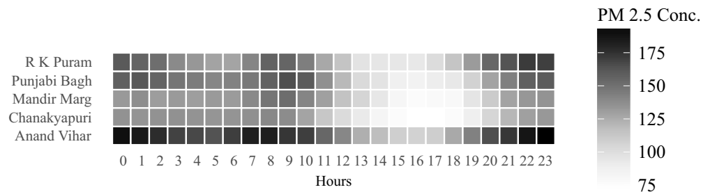
Fig 3. Month effects in pollution levels.
