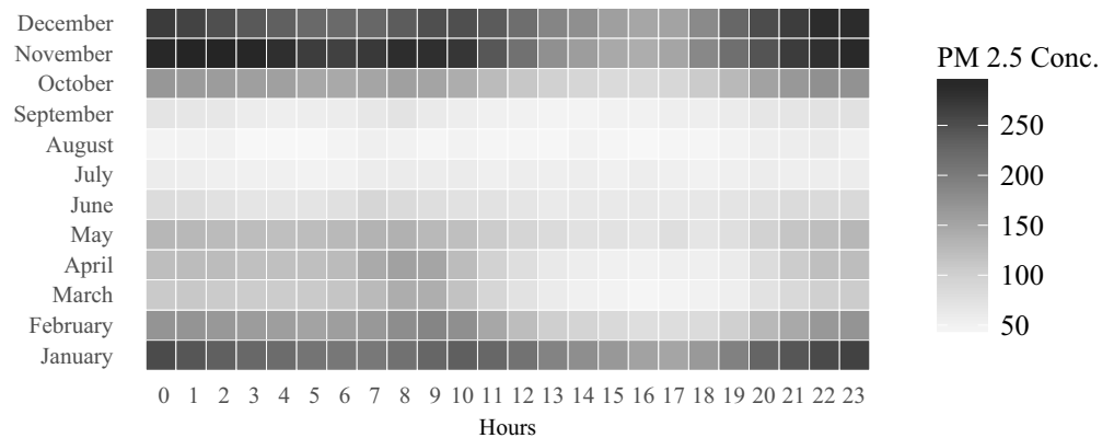
Fig 2. Location effects in pollution levels.
