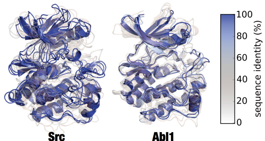
Fig 7. Superposition of clustered models of Src and Abl1. Superposed renderings of nine models each for Src and Abl1, giving some indication the diversity of conformations generated by Ensembler. The models for each target were divided into three sequence identity ranges (as in Fig 5), and RMSD-based k -medoids clustering was performed (using the msmbuilder clustering package [18]) to select three clusters from each. The models shown are the centroids of each cluster. Models are colored and given transparency based on their sequence identity, so that high sequence identity models are blue and opaque, while lower sequence identity models are transparent and red.
