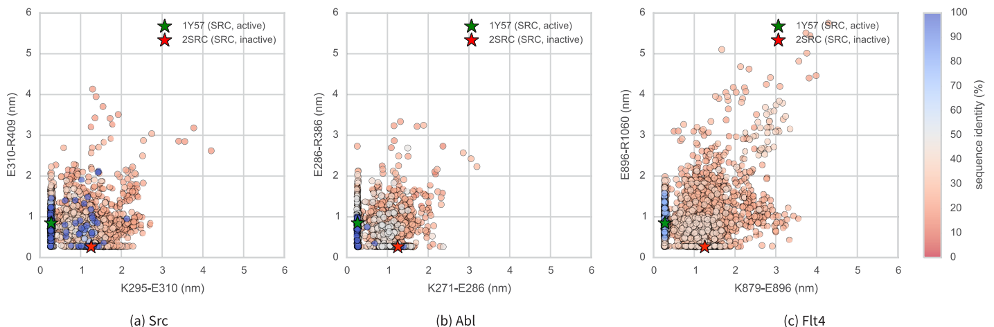
Fig 9. Src, Abl1, and Flt4 models projected onto the distances between two conserved residue pairs, colored by sequence identity. Two Src structures (PDB entries 1Y57 [57] and 2SRC [56]) are projected onto the plots for reference, representing active and inactive states respectively. These structures and the residue pairs analyzed here are depicted in Fig 8 . Distances are measured between the center of masses of the three terminal sidechain heavy atoms of each residue. The atom names for these atoms, according to the PDB coordinate files for both reference structures, are—Lys: NZ, CD, CE (ethylamine); Glu: OE1, CD, OE2 (carboxylate); Arg: NH1, CZ, NH2 (part of guanidine).
