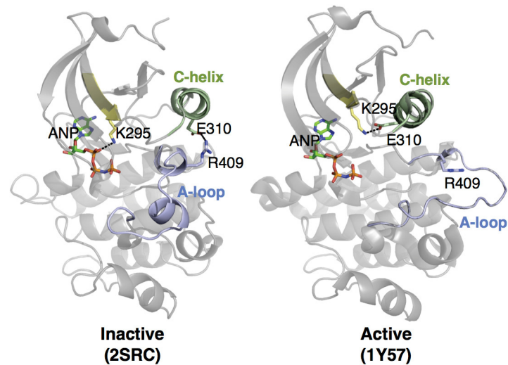
Fig 8. Two structures of Src, indicating certain residues involved in activation. In the inactive state, E310 forms a salt bridge with R409. During activation, the \alpha C-helix (green) moves and rotates, orienting E310 towards the ATP-binding site and allowing it to instead form a salt bridge with K295. This positions K295 in the appropriate position for catalysis. Note that ANP (phosphoaminophosphonic acid-adenylate ester; an analog of ATP) is only physically present in the 2SRC structure. To aid visualization of the active site in 1Y57, it has been included in the rendering by structurally aligning the surrounding homologous protein residues.
