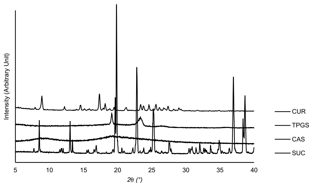
Figure 5 XRD pattern of curcumin and single components used in the developed MC-SDP formulations.
