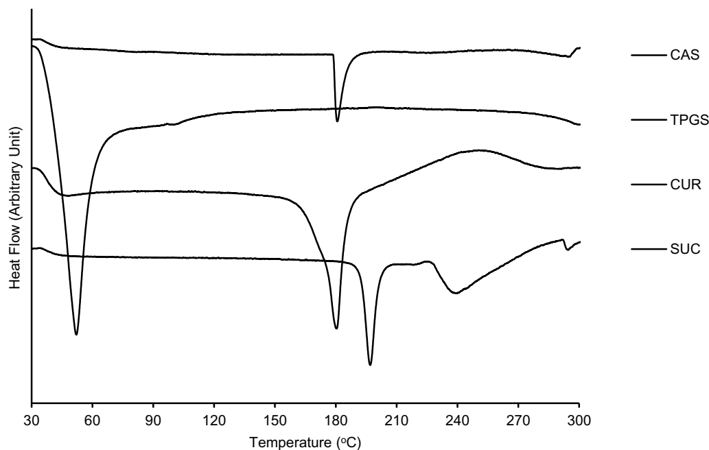
Figure 3 DTA thermograms of curcumin and single components used in the developed MC-SDP formulations.
