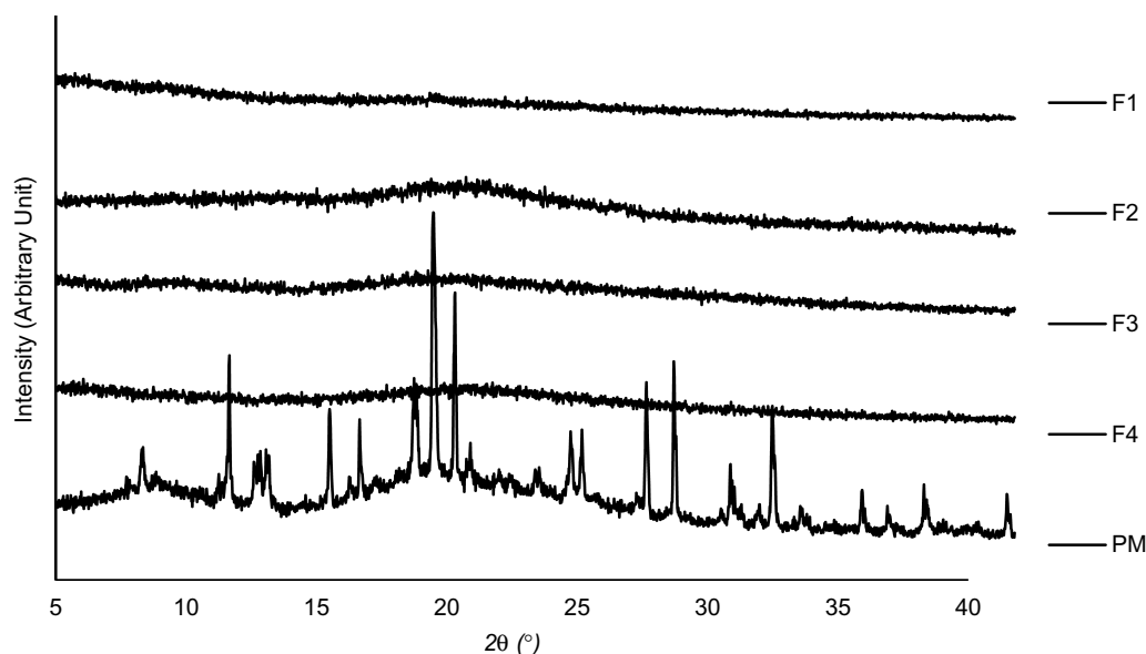
Figure 6 XRD patterns of MC-SDPs containing curcumin made at different percentage weight ratios of CAS:TPGS:SUC and their physical mixture.
