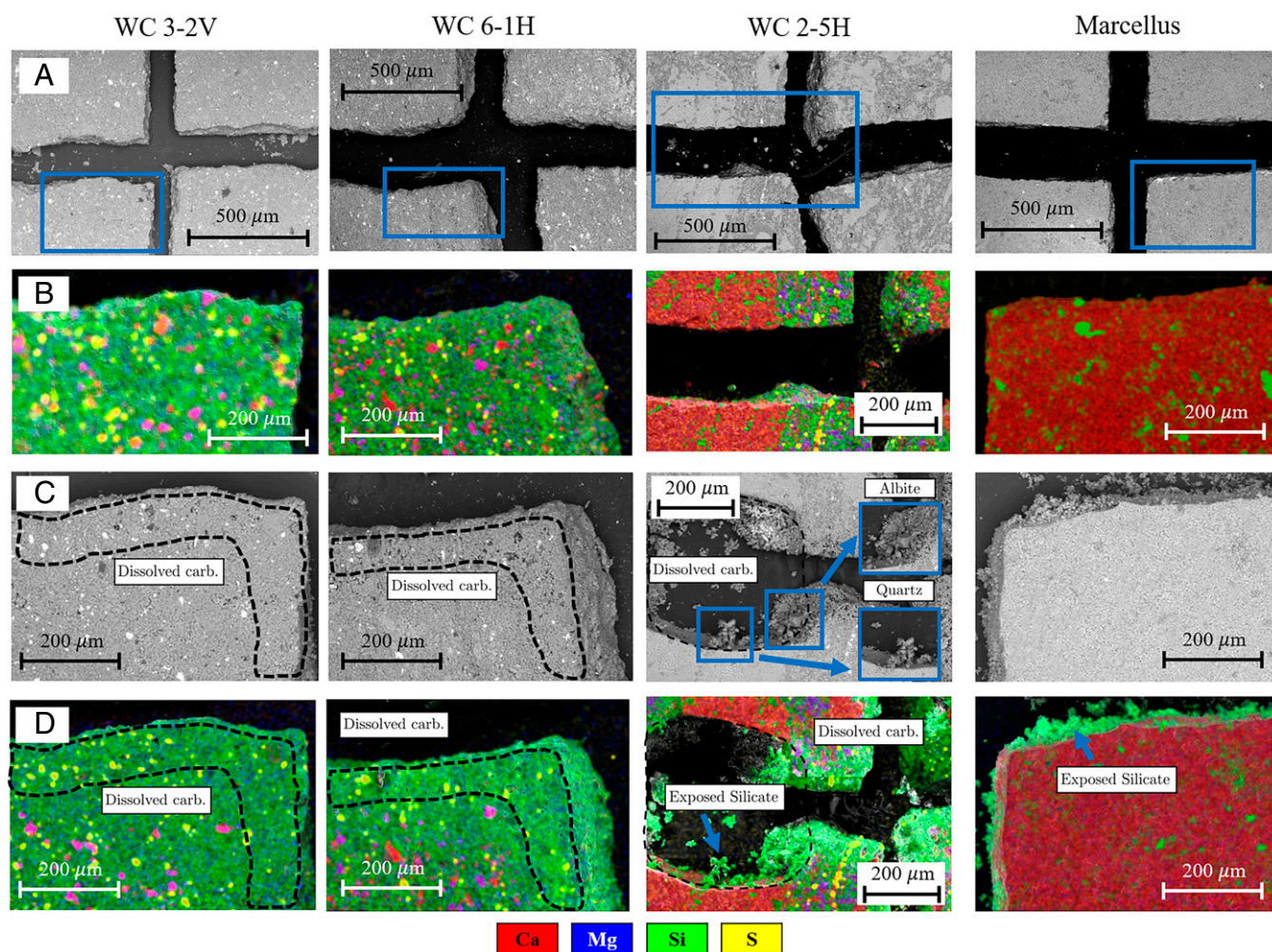
Fig. 4. (A) Prereaction SEM-BSE images of the four samples (image width = 1.38 mm). Blue boxes (image width ~0.5 mm) correspond to select regions of prereaction EDS, postreaction SEM-BSE, and postreaction EDS images in B–D . (B) Prereaction composite elemental maps for the select region. (C) Postreaction SEM-BSE images of the same region. Insets show albite and quartz crystals exposed after the dissolution of surrounding calcite. (D) Corresponding postreaction composite elemental maps. Samples are ordered from carbonate-poor on the left to carbonate-rich on the right. The carbonate dissolution zones with newly developed porosity are indicated by dashed lines. The dashed region for WC 2-5H corresponds to calcite dissolved from both sides of the fracture. In this sample, calcite dissolution exposed euhedral quartz and albite. Fine-grained silicates are also exposed by calcite dissolution in the Marcellus sample. The colors indicate individual elements as listed for each composite element image. Full-size composite elemental images and SEM-BSE images are in SI Appendix, Fig. S4–S7 . These images along with single element maps are available in the Stanford Digital Repository (see Data Availability ).
