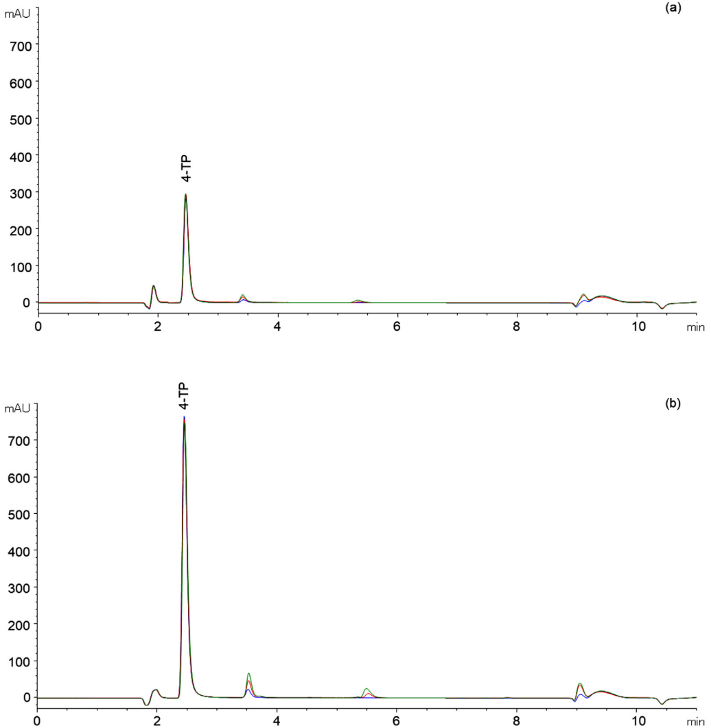
Fig. 5. Chromatograms of \beta -Lg solutions ( 9 \text{ g L}^{-1} ) for quantification of free (a) and total (b) thiols as a function of the DTDP [ \mu\text{mol} ]/thiol expected [ \mu\text{mol} ] concentration ratio (0.5/1 (blue), 1.1/1 (red), 1.6/1 (green)).
