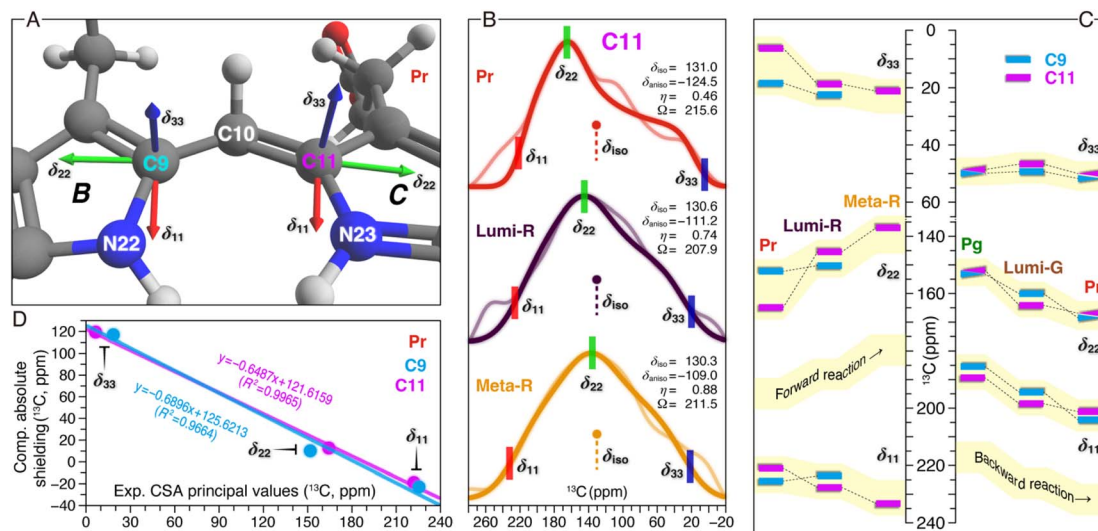
Fig. 5 ^{13}\text{C} CSA tensor values of C9 and C11 in both reaction pathways. (A) Calculated orientations of the principal axes on the molecular frame of C9 (connecting N22 of ring B and C10) and C11 (connecting N23 of ring C and C10). For calculation details of the CSA tensors, see ESI, Experimental.† (B) SUPER pseudostatic powder patterns of C11 in the Pr state and the two intermediates of the forward-reaction, Lumi-R and Meta-R (thin lines) with best-fit simulations (thick lines). The applied line broadening for the three simulated spectra of Pr, Lumi-R, and Meta-R was 200, 300, and 350 Hz, respectively. For each photocycle state, the isotropic value ( \delta_{\text{iso}} in ppm, defined as (\delta_{11} + \delta_{22} + \delta_{33})/3 ), anisotropy parameter ( \delta_{\text{aniso}} in ppm, defined as |\delta_{11} - \delta_{\text{iso}}| for describing the largest separation from the center of gravity of the line shape), asymmetry parameter ( \eta , defined as (\delta_{22} - \delta_{33})/\delta_{\text{aniso}} indicating how much the line shape deviated from that of an axially symmetric tensor), and span ( \Omega in ppm, defined as |\delta_{11} - \delta_{33}| for describing the maximum width of the powder pattern) are indicated. The best-fit uncertainties are \pm 1.2 ppm for \delta_{\text{aniso}} and \pm 0.05 for \eta . (C) Changes in the three experimental principal values of C9 and C11 during the Pr \rightarrow Lumi-R and Lumi-R \rightarrow Meta-R transitions of the forward-reaction are shown (left panel). For C9 only the changes associated with the Pr \rightarrow Lumi-R transition are determined (for line shape analysis, see Fig. S7†). Calculated principal values are shown for Pg, Lumi-G, and Pr in the backward-reaction (right panel). All CSA principal values are summarized in Tables S4–S6.† (D) Correlations between the calculated and experimental principal values of the chemical shift tensors for C9 (cyan) and C11 (magenta) in the Pr state. The equations from linear regression and corresponding R^2 coefficients are shown in the inset.
