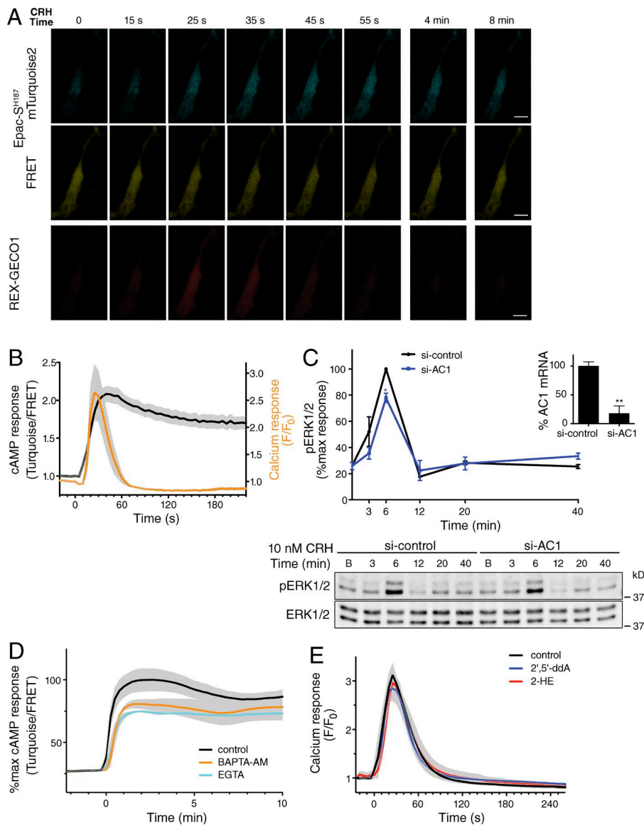
Figure 7. CRH-triggered calcium response regulates cAMP. (A and B) HT22-CRHR1 cells cotransfected with Epac-SH 187 and REX-GECO1 were stimulated with 100 nM CRH. (A) Representative images for each signal. Bar, 5 \mu m. (B) Time course of FRET changes (black trace) or REX-GECO1 fluorescence (orange trace). Data: mean \pm SEM, 14 cells. (C) pERK1/2 and total ERK1/2 were measured in HT22-CRHR1 cells transfected with 50 nM siRNA against GL3 (control) or AC1 and stimulated with CRH. Results are expressed as the percentage of maximum pERK1/2 after stimulation under control conditions (mean \pm SEM, n = 3 ). *, P < 0.05 ; **, P < 0.01 by Student's t test. Efficiency of AC1 knockdown assessed by quantitative RT-PCR normalized to HPRT is shown (mean \pm SEM, n = 3 ). **, P < 0.01 by Student's t test. (D) HT22-CRHR1-Epac-SH 187 cells preincubated with vehicle (control), 5 \mu M BAPTA-AM, or 500 \mu M EGTA were stimulated at time 0 with CRH. Time course of FRET changes was measured in single cells (mean \pm SEM, n = 3 ). (E) Calcium response was determined in HT22-CRHR1 cells pretreated with tmAC-specific (100 \mu M ddA) or sAC-specific (20 \mu M 2-HE) inhibitors, loaded with Fluo-4-AM, and stimulated at time 0 with 100 nM CRH (mean \pm SEM, n = 3 ).
