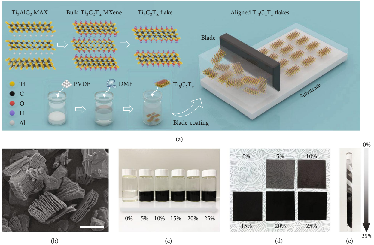
FIGURE 1: Design and synthesis of the MXene-embedded PVDF membrane. (a) Schematic illustration of the formation procedure of the Ti_3C_2T_x MXene flakes (etching and ultrasonication) and the preparation of the MXene-embedded PVDF membrane by blade coating. (b) Scanning electron microscopy (SEM) image of the fabricated MXene flakes. Scale bar, 5 \mu m. (c) Digital photographs of the MXene/PVDF composite solution with different doping content of MXene ranging from 0% to 25%. (d, e) Images of the prepared MXene-embedded PVDF membrane with different doping content.
