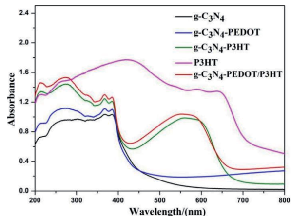
Fig. 4 UV-Vis diffuse reflectance spectra of the g\text{-C}_3\text{N}_4\text{-polymer} samples.
