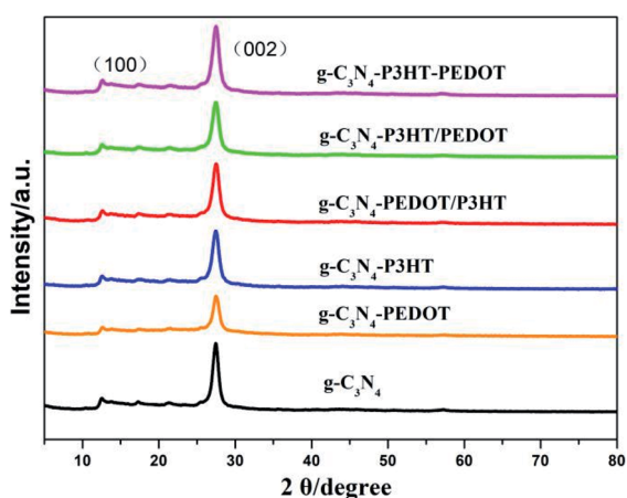
Fig. 2 XRD patterns of the as-prepared g\text{-C}_3\text{N}_4\text{-polymer} samples.
