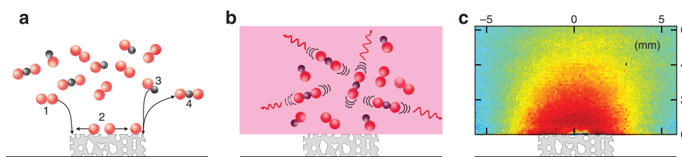
Figure 1 | Schematic of planar laser-induced fluorescence. Schematic of PLIF measurements of the activity of a model catalyst (a) shows the adsorption and dissociation of O 2 on the catalyst at points 1 and 2, respectively, and the adsorption of CO and production of CO 2 at points 3 and 4, respectively. (b) The laser sheet (pink) that excites the CO 2 molecules above the catalyst; the fluorescence from the excited molecules is detected. An example of the CO 2 distribution above an active catalyst at elevated temperature and realistic pressure is shown in c.
