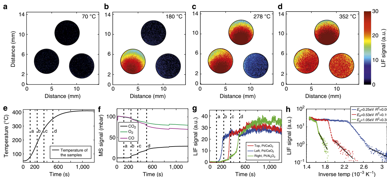
Figure 4 | The CO 2 signal from three different samples in three separate exhaust tubes. (a–d) The CO 2 signal from the gas exiting the three tube ends are shown in the top panel (see Supplementary Movie 4). (e) The temperature measured by the thermocouple located centred between the tubes at the same position as the samples, (f) the MS signal during the event and (g) the averaged infrared PLIF signal exiting each tube, which is also shown in three Arrhenius plots in h.
