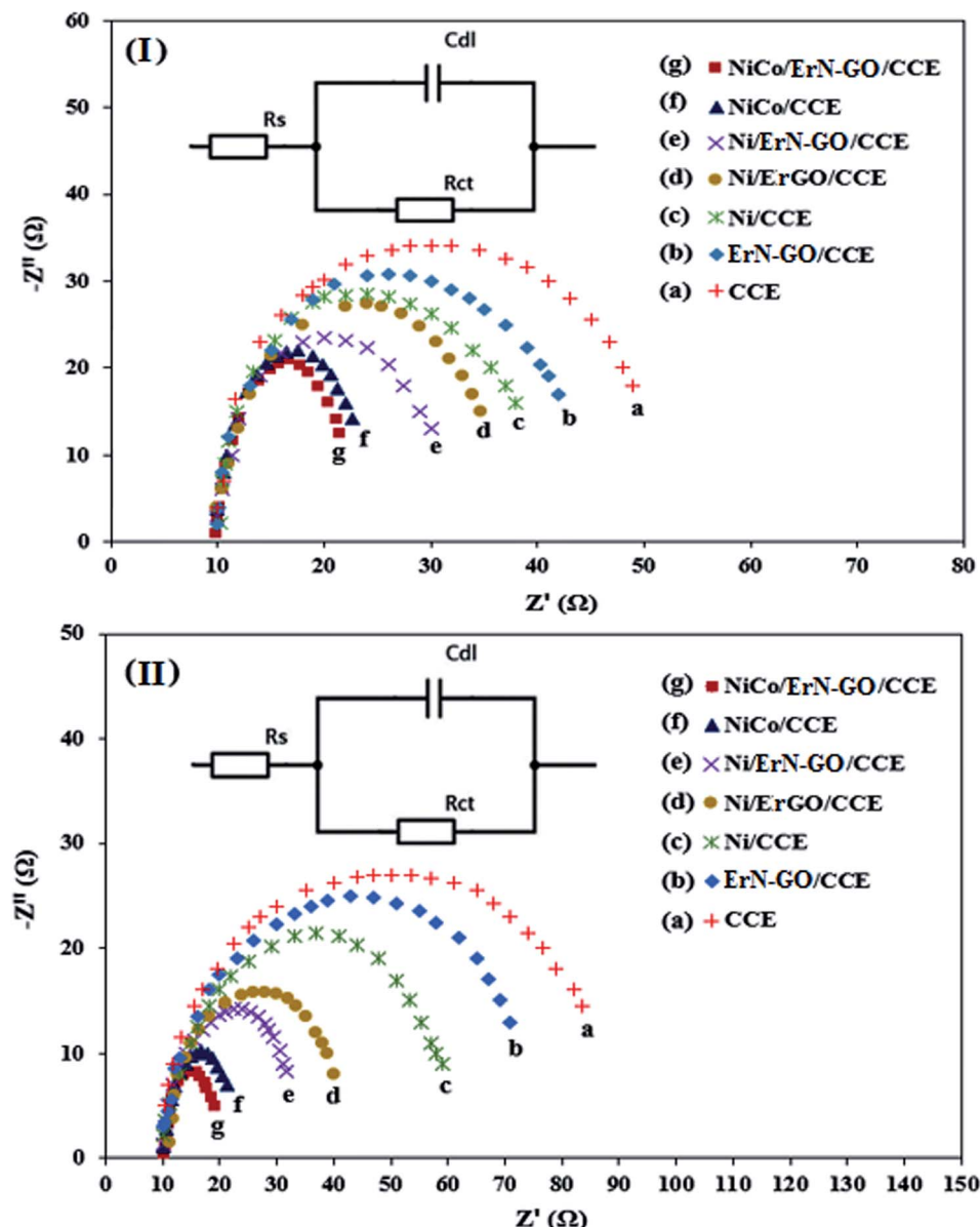
Fig. 12 Nyquist plots of impedance measurements (at 0.6 V vs. Ag/AgCl) in 0.1 M KOH + 0.1 M methanol solution (I) and 0.1 M KOH + 0.1 M ethanol solution (II) on the (a) CCE, (b) ErN-GO/CCE, (c) Ni/CCE, (d) Ni/ErGO/CCE, (e) Ni/ErN-GO/CCE, (f) NiCo/CCE and (g) NiCo/ErN-GO/CCE. Insets are the Randles equivalent circuit for NiCo/ErN-GO/CCE.
