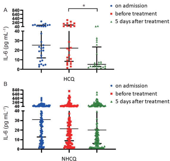
Figure 2 Effects of HCQ treatment on plasma levels of IL-6. HCQ treatment significantly decreased the levels of IL-6 in about 5 (4–8) days, * P < 0.05 (A). The levels of IL-6 were not significantly decreased in NHCQ treatment group at the same observation time (B). Data are presented as medians and interquartile range (Q1–Q3).
