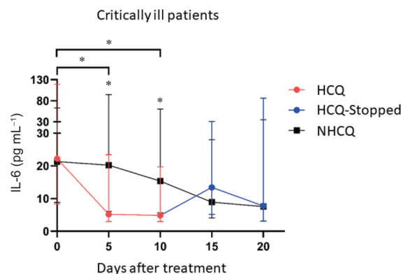
Figure 3 Continuous curves of plasma levels of IL-6 showing that the consistency of HCQ treatment period with lowering IL-6 levels, * P < 0.05 . Data are presented as medians and interquartile range (Q1–Q3).
