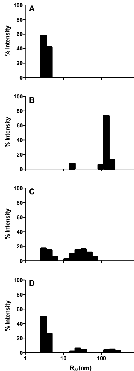
Figure 4 Effect of BSA inhibition of A\beta_{1-40} monomer aggregation on aggregate size distribution. A\beta_{1-40} monomer aggregations were performed as in Figure 1 for 20 \mu M A\beta_{1-40} monomer in the presence of 0 \mu M (panel B, control), 40 \mu M (panel C), or 80 \mu M (panel D) BSA. In addition, 80 \mu M BSA was subjected to aggregation conditions in the absence of A\beta_{1-40} monomer (panel A). DLS was employed to determine R_H distributions. Results are presented as intensity-weighted histograms derived from data regularization with Dynamics Software (Wyatt Technology). Results are representative of two independent experiments.
