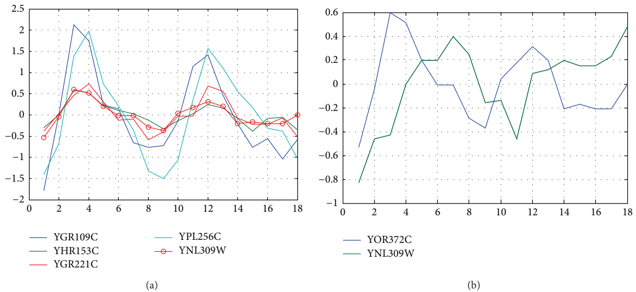
FIGURE 5: Coexpression analysis of yeast cell-cycle transcription factor YNL309W. (a) GESearch detected four cell-cycle target genes, including the known targets YGR109C, YPL256C, and YGR221C, and the newly detected YHR153C. (b) The target gene of YOR372C was in shifted expression profiles, which was not detected by GESearch, but was identified by the time delay analysis.
