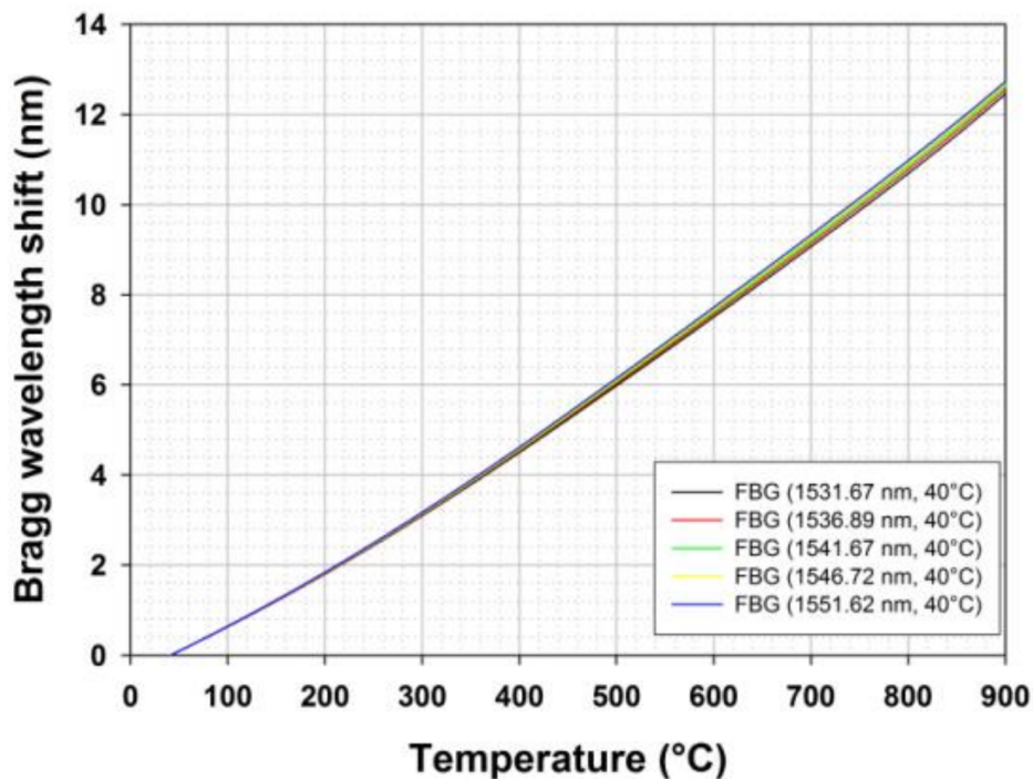
Figure 3. Bragg wavelength shift with temperature up to 900 °C for five regenerated FBGs realized and calibrated at CEA List laboratory. The seed FBGs were written using a 244 nm continuous-wave Argon Ion laser (Fred Innova 300C from Coherent) into H 2 -loaded smf-28 optical fibre. Regeneration was performed at 910 °C in a tubular furnace.
