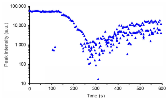
Figure 9. Regeneration of FBG using CO 2 laser annealing. Annealing parameters: scan movement: sinus + gating signal, f_{SCAN} = 100 Hz, DX_{SCAN} = 14 mm, PWM < 40%, f_{CO_2} = 20 kHz.
