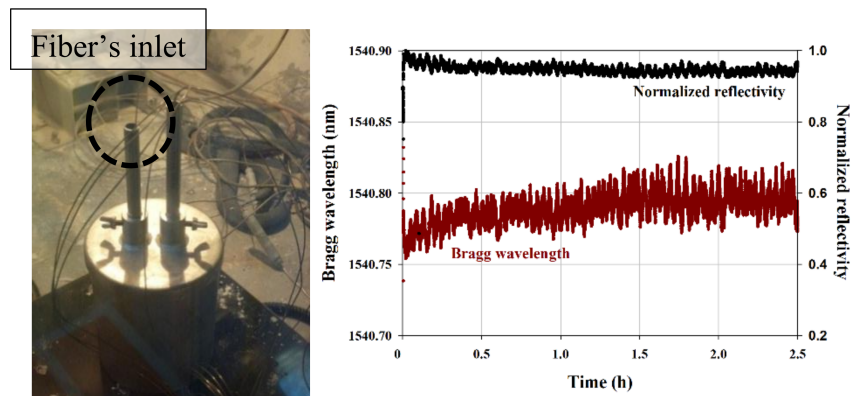
Figure 13. Sodium box installed in the Penelope facility and heated from the bottom (left). The fiber's inlet is highlighted: a single capillary is enough to position 5 multiplexed regenerated FBGs; the other inlet is for three thermocouples. On the right, stability of a regenerated FBG in hot sodium ( 500^\circ\text{C} ).
