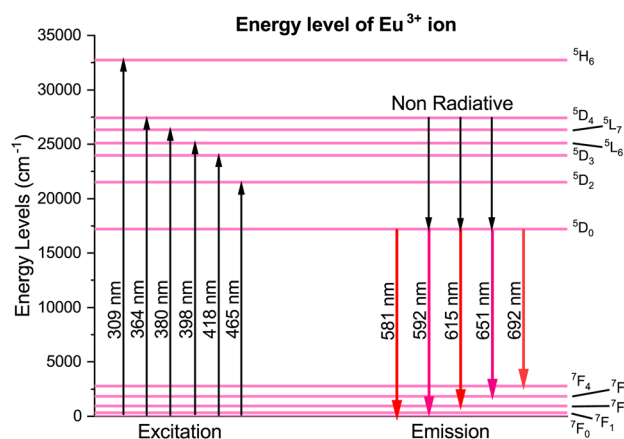
Fig. 18 Partial energy-level diagram of \text{Eu}^{3+} in the \text{Na}_3\text{Ba}_2\text{LaNb}_{10}\text{O}_{30} phosphor.
