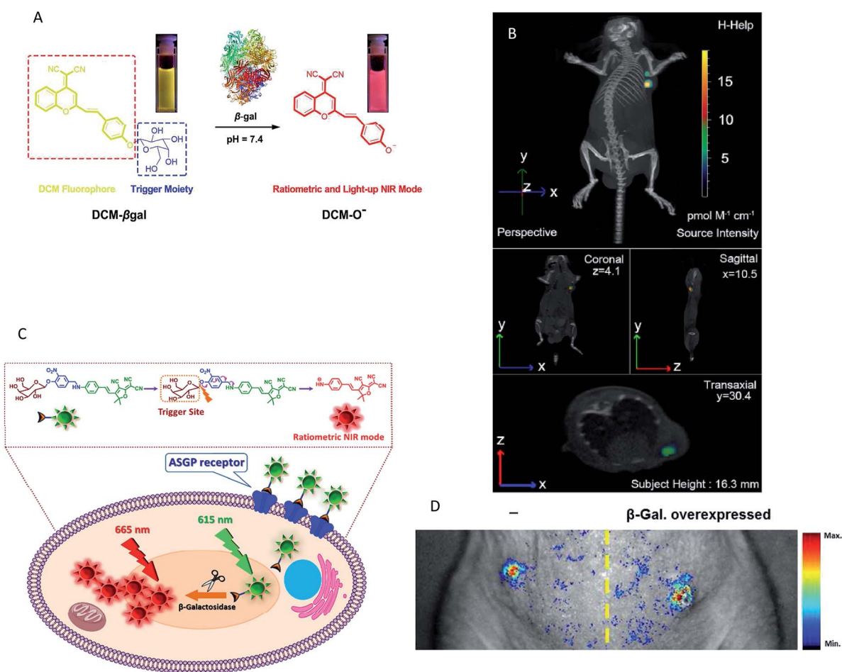
Fig. 3 (A) Conceptual scheme of β-Gal enzymatic activation of DCM-βgal. (B) Three-dimensional in vivo imaging of DCM-βgal. (C) Conceptual scheme of DCDHF-βgal when encountering β-Gal and the following fluorescence change. (D) In vivo fluorescence imaging of DCDHF-βgal. (A and B) Reproduced from ref. 54. Copyright 2016 American Chemical Society. (C and D) Reproduced from ref. 53. Copyright 2017 Elsevier.
