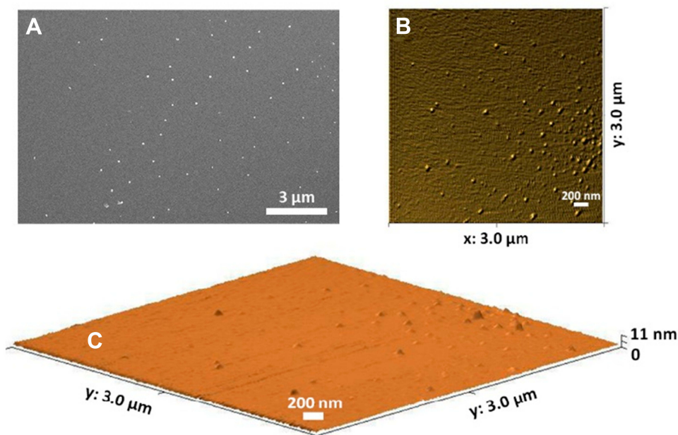
Figure 2 Morphology analysis of prepared DPs by microfluidic platform at the N/P ratio of 10, (A) Representative field emission scanning electron microscopy (FESEM), scale bar 3 μm, (B) Surface topography of DPs, 2D AFM imaging, (C) 3D AFM imaging, scan size 3×3μm.
