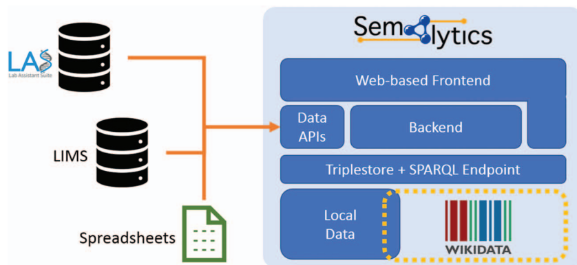
Figure 6. Deployment of Semalytics as a Web-based platform. Local data are mapped to Wikidata creating an annotation system with extended knowledge. Those two data spaces can be federated with SPARQL. The backend and the Web frontend help users interact with data, even if they are not familiar with SPARQL query language. Finally, data Application Programming Interfaces manage information ingestion from external sources (e.g. LIMSs or spreadsheets), as well as the exporting of results of local data processing. Those two data spaces can be federated with SPARQL. The backend and the Web frontend help users interact with data, even if they are not.
