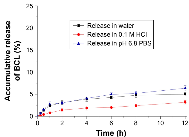
Figure 4 Release profiles of BCL from nanoemulsions with the time in water, 0.1 M HCl, and PBS, pH 6.8 (n=3, mean ± StD).
